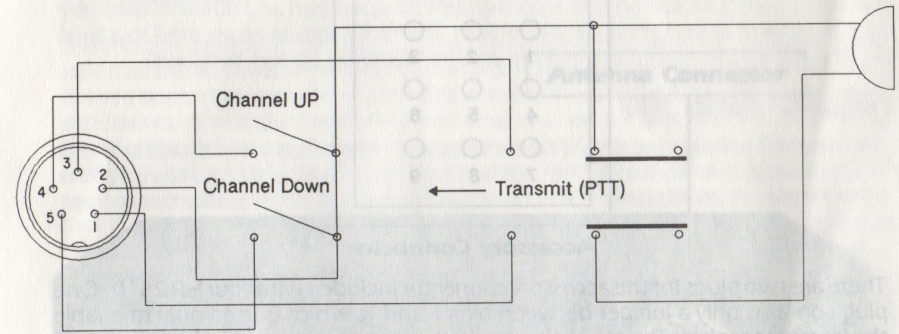
Microphone Connector
